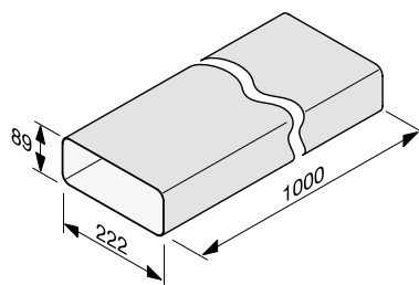
Flatkanal DFK-R 1000
