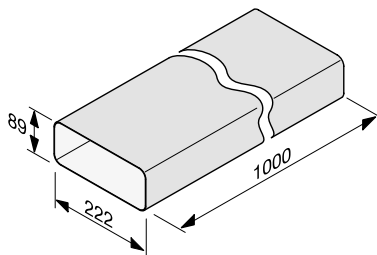
Flatkanal DFK-R 1000
