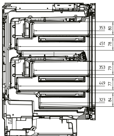
KWT 6322 UG – Interior cabinet
