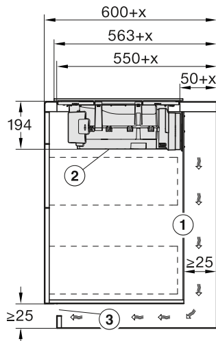
KMDA 7272 FR, KMDA 7473 FR Frame – Surface-mounted installation
