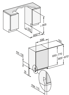
Fully integrated dishwashers, 60 cm wide
