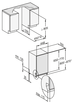
Fully integrated dishwashers, 45 cm wide
