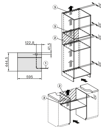
DG 7000, DGM 7000, 24 l oven compartment
