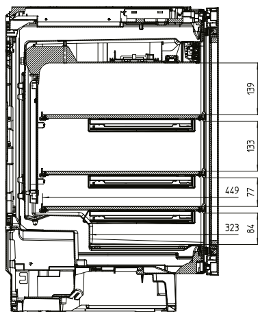
KWT 6312 UGS – Interior cabinet
