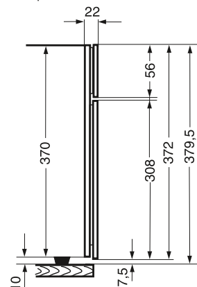
DG 6001, DG 6019, 24 l oven compartment
