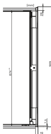
KWT 6422 iG – Side view
