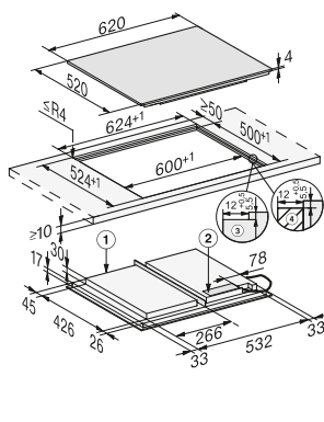
KM 7667 FL Flush-fit installation
