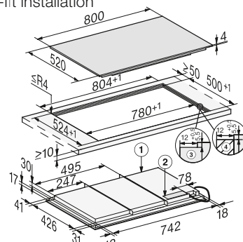
KM 7678 FL, KM 7878 FL, KM 7878-1 FL Diamond, KM 7878-2 FL Diamond Flush-fit installation
