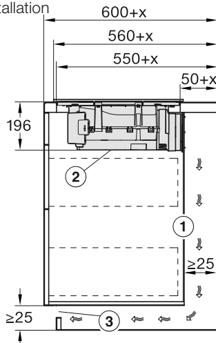
KMDA 7272 FL, KMDA 7473 FL Frameless – Surface-mounted installation
