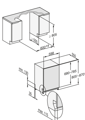
Fully integrated dishwashers, 60 cm wide, FrontFit
