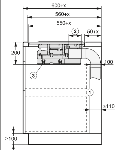
KMDA 7476 FL, KMDA 7634 FL Frameless – Flush-fit installation
