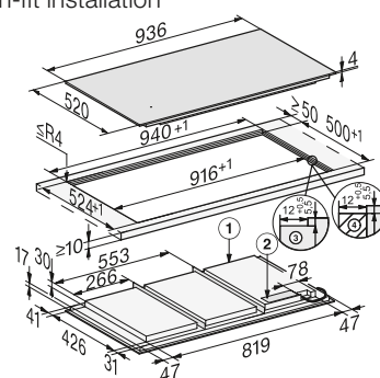
KM 7697 FL, KM 7897 FL, KM 7897-1 FL Diamond, KM 7897-2 FL Diamond Flush-fit installation
