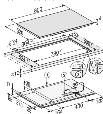
KM 7574 FL Flush-fit installation
