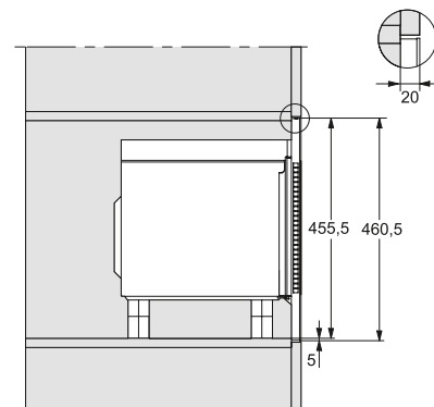
M 2240, 46 l oven compartment
