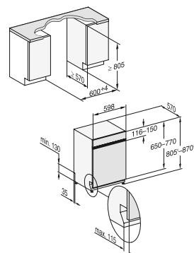
Semi-integrated dishwashers, 60 cm wide
