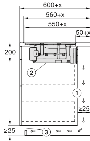
KMDA 7272 FL, KMDA 7473 FL Frameless – Flush-fit installation
