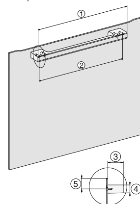
Handle DG 7000, DGM 7000, 24 l oven compartment PureLine
