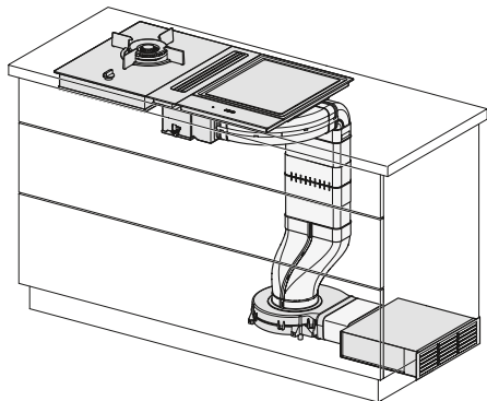
Gaine plate DFK-R 1000
