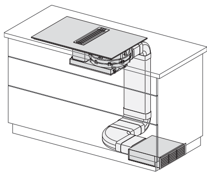
Fladkanal DFK-R 1000
