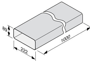
Fladkanal DFK-R 1000
