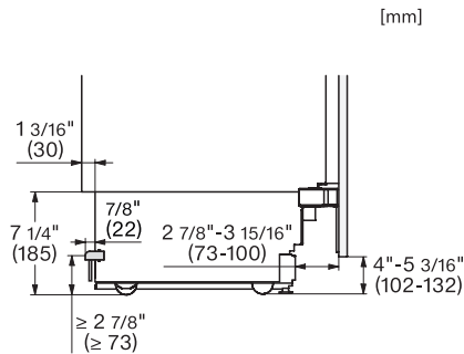
KFMC3642FD, KFMC3844FD, MasterCool III, integration, panel ready
