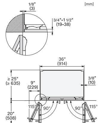
KFMC3642FD, KFMC3844FD, MasterCool III, panel ready, top view
