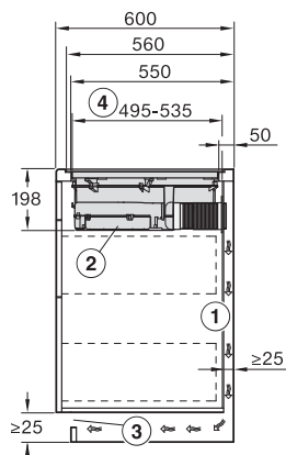
KMDA5649FL, KMDA5649FR, KMDA5649FL MattFinish – Installation variant 10 Exhaust air
