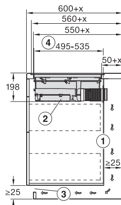
KMDA5649FL, KMDA5649FR, KMDA5649FL MattFinish – Installation variant 12 Exhaust air
