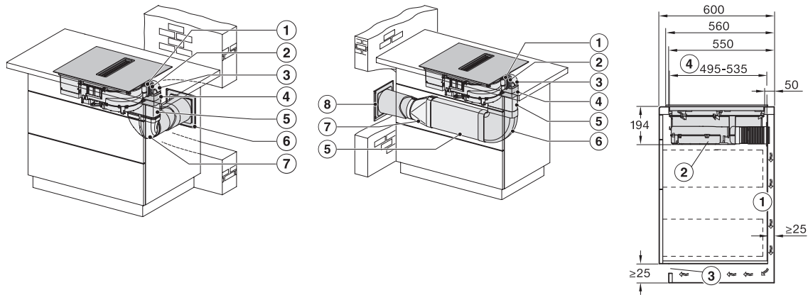
KMDA5649FL, KMDA5649FR, KMDA5649FL MattFinish – Installation variant 10 Exhaust air
