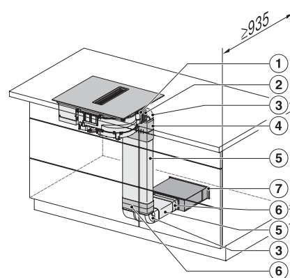
KMDA5649FL, KMDA5649FR, KMDA5649FL MattFinish – Installation variant 6 Circulating air
