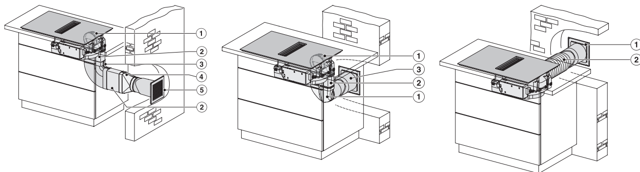
KMDA7676-1FL, KMDA7876-1FL, KMDA7676FL, KMDA7876FL – Installation variant 9 Exhaust air
