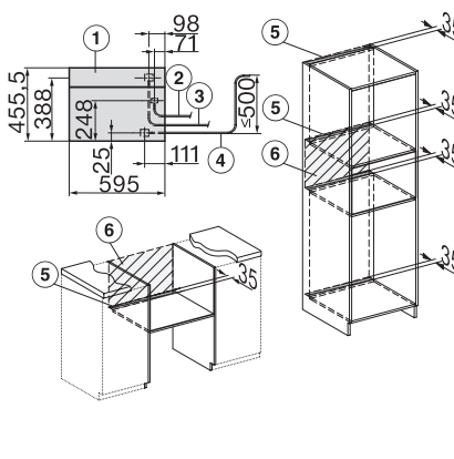
DGC7x45 connections and ventilation 45cm, installation drawing
