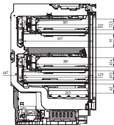
KWTUS7074F, interior dimensions (installation drawings)
