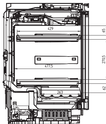
KWTUS7055F, interior dimensions (installation drawings)
