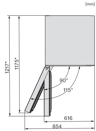
FNS4782E bb Blackboard, top view (*footnote) (installation drawings)
