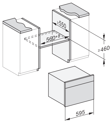
DGC7x4x, DGC7x4x installation drawings
