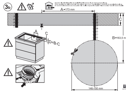
KMDA7676-1FL, KMDA7876-1FL – flush, drilling template, Installation depth 23,8 cm
