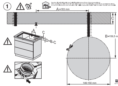
KMDA7676-1FL, KMDA7876-1FL, KMDA7676FL, KMDA7876FL – Installation variant 12 Exhaust air
