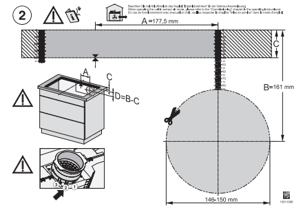
KMDA7676-1FL, KMDA7876-1FL, KMDA7676FL, KMDA7876FL – Installation variant 13 Circulating air
