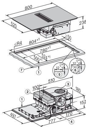
KMDA7676-1FL, KMDA7876-1FL, KMDA7676FL, KMDA7876FL – flush
