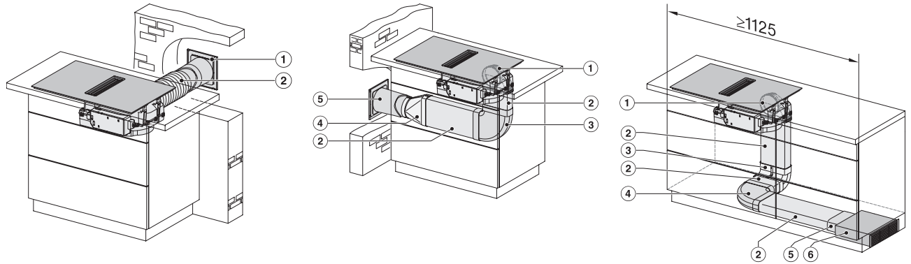
KMDA7676-1FL, KMDA7876-1FL, KMDA7676FL, KMDA7876FL – Installation variant 11 Exhaust air
