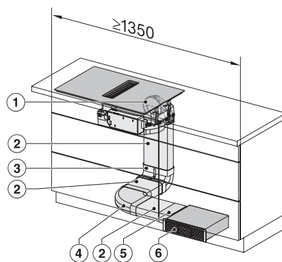
KMDA7676-1FL, KMDA7876-1FL, KMDA7676FL, KMDA7876FL – Installation variant 4 Circulating air
