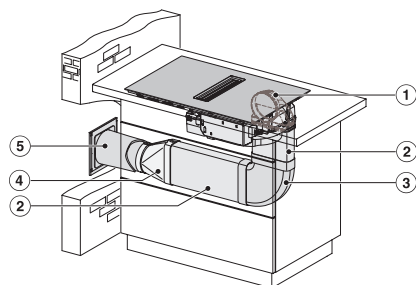
KMDA7272-1FL/FR, KMDA7473-1FL/FL MattFinish/FR, KMDA7272FL/FR, KMDA7473FL/FR – Installation variant 9 Exhaust air
