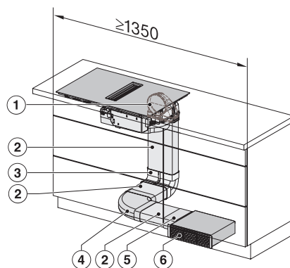
KMDA7272-1FL/FR, KMDA7473-1FL/FL MattFinish/FR, KMDA7272FL/FR, KMDA7473FL/FR – Installation variant 4 Circulating air
