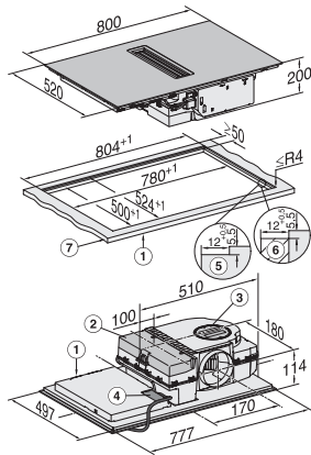
KMDA7272-1FL, KMDA7272FL, KMDA7473FL, KMDA7473-1FL – flush
