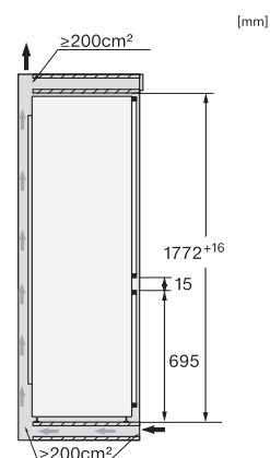
KFNS7734D, KFN7734C, KFN7734F, KFN7734D, KFN7764D, KFN7785D, KFN7744E, KFN7774B, side view
