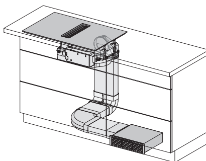
KMDA7676-1FL, KMDA7876-1FL, KMDA7676FL, KMDA7876FL – Installation variant 6 Circulating air
