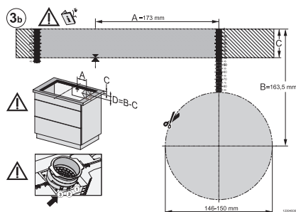
KMDA7676FL-U, KMDA7876FL-U – flush, drilling template, Installation depth 23,8 cm
