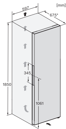
K4373DD, K4373ED, FN4372E, FN4372D, installation sketch
