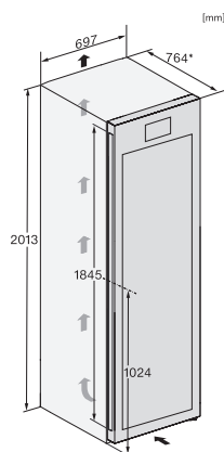
KWT4999F obsw, KWT4995F obsw, Rioja, installation sketch
