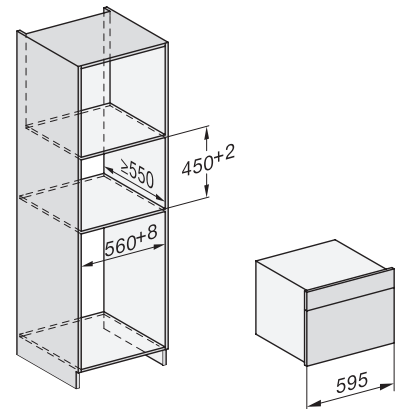
DG DGM, installation drawing
