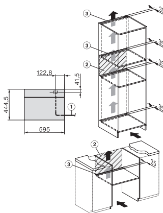
Installation DG, installation drawing
