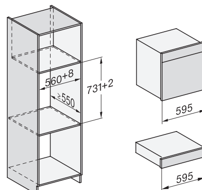
Installation_DGC_XXL_ESW7x10_EVS7010 installation drawings
