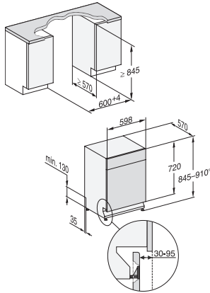
G7000, built under, XXL, dishwasher, 60cm (installation drawing)
