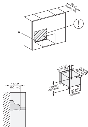
M2241SC, Installation, 30 Zoll, Proud, Oberschrank – Skizze – NA
