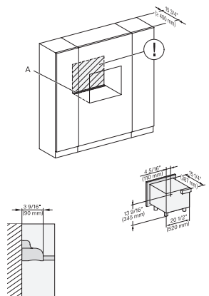
M2241SC, Installation, 30 Zoll, Proud, breite Front – Skizze – NA
