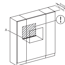
M7240TC+EBA7848, Einbau, 30 Zoll, Proud, built-under, wide front
