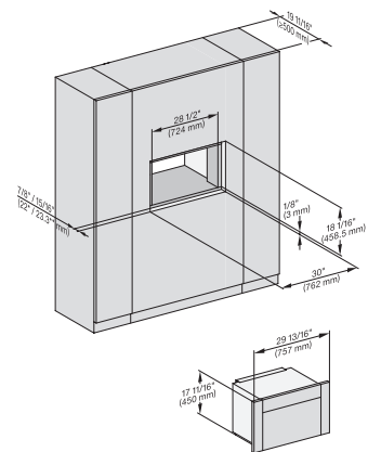
M7240TC+EBA7848, Einbau, 30 Zoll, Flush inset, wide front
