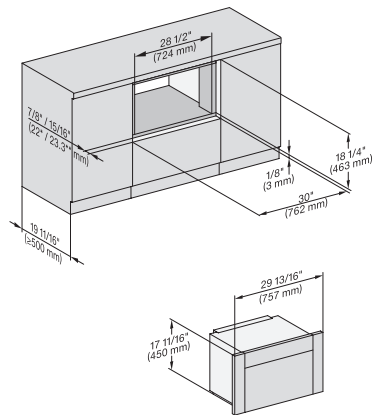
M7240TC+EBA7848, Einbau, 30 Zoll, Flush inset, built-under
