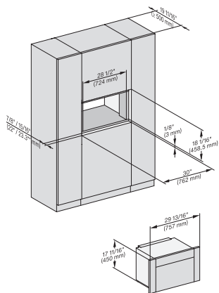
M7240TC+EBA7848, Einbau, 30 Zoll, Flush inset
