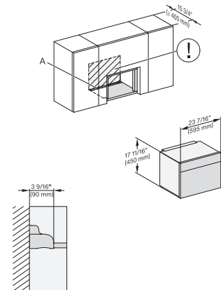
M7240SC(+EBA7848), Installation, 30 Zoll, Flush, inset, breite Front, Oberschrank – Skizze – NA
