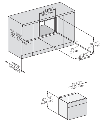
M7240TC, Einbau, 30 Zoll, Flush Inset, built-under, wide front
