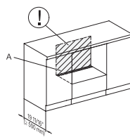
M7240TC, Einbau, 30 Zoll, Proud, built-under, wide front
