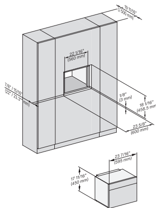
M7x4xTC, Einbau, 30 Zoll, Flush inset, wide front
