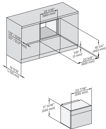
M7240TC, Einbau, 30 Zoll, Flush inset, built-under
