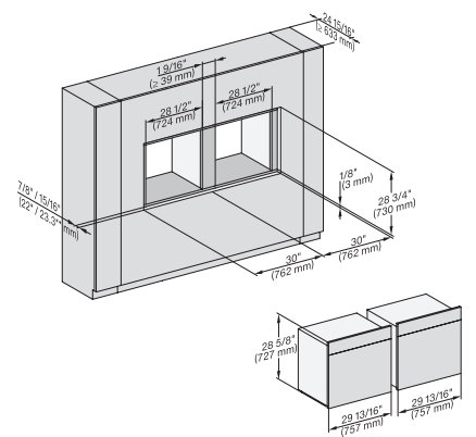
H 6x80 BP, H 6x80-2BP, H 2x80BP, H 7x80 BP/BPX Fitting Combi wide front side by side, Install. drawing, Flush inset, NA
