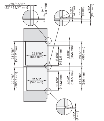
DGC6x6x(AM)+EBA6808, H6560B+EBA6808, H6x60BP+EBA6808, (DGC786x, H7x6xBP)+EBA7868, Combi, Installation drawing, Proud, NA
