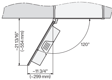
CVA7445, CVA7845, side view, 60 cm, Proud
