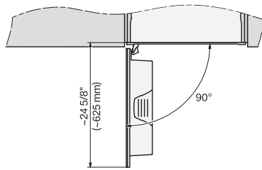
CVA7000, installation (installation drawings)
