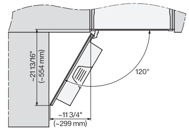
CVA7440, CVA7445, CVA7840, CVA7845, installation drawing, view from above, 60 cm, Flush inset
