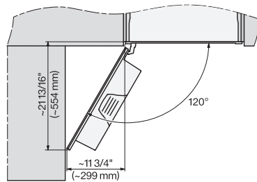
CVA7440, CVA7445, CVA7840, CVA7845, installation drawing, view from above, 60 cm, Flush inset
