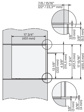
CVA7440, CVA7840, installation drawing, side view, Flush inset
