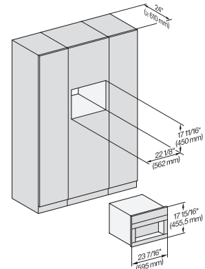
CVA7440, CVA7445, CVA7840, CVA7845, installation drawing, built in, Einbau, 60 cm, Proud
