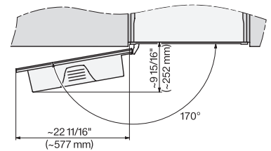
CVA7440, CVA7445, CVA7840, CVA7845, installation drawing, view from above, 60 cm, Flush inset
