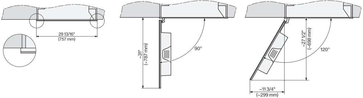
CVA7370, CVA7775, CVA7875, installation drawing, view from above, 30 Inch, Proud
