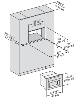
CVA7370, CVA7775, CVA7875, installation drawing, built in, 30 Inch, Flush inset
