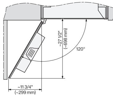
CVA7370, CVA7775, CVA7875, installation drawing, view from above, 30 Inch, Flush inset
