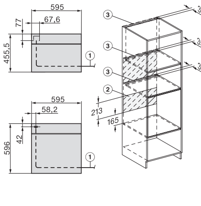
Installation Kombi BM XL, installation drawings
