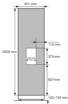
KFP1240ss, dimensions of furniture fronts F1471Vi, F1472Vi, MasterCool (Sketch)
