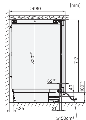
KWTUS7096E, Built-under, side view
