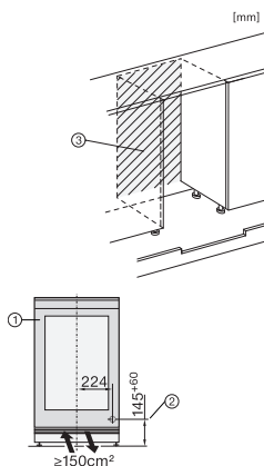
KWTUS7054F, KWTUS7055F, KWTUS7074F, KWTUS7096E, KWTUS7196E, Built-under, side view (*footnote)
