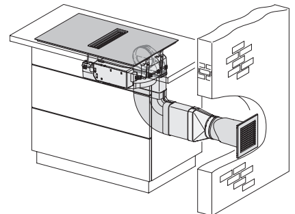
KMDA7676-1FL, KMDA7876-1FL, KMDA7676FL, KMDA7876FL – Installation variant 10 Exhaust air
