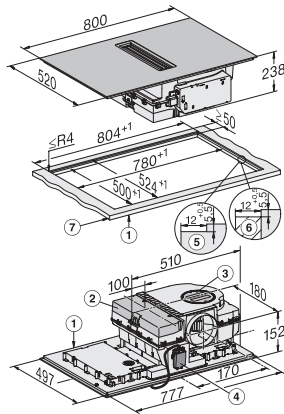
KMDA7676-1FL, KMDA7876-1FL, KMDA7676FL, KMDA7876FL – flush
