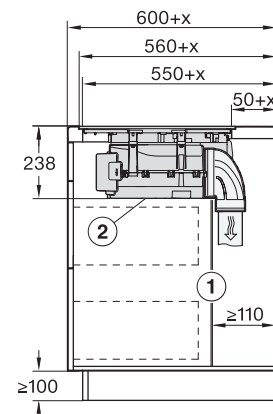
KMDA7676-1FL, KMDA7876-1FL, KMDA7676FL, KMDA7876FL – Side view flush+X
