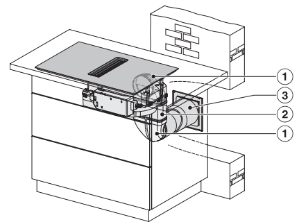
KMDA7676-1FL, KMDA7876-1FL, KMDA7676FL, KMDA7876FL – Installation variant 2 Basis
