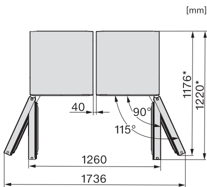
K4373ED, KS4383ED, KS4383 C ED, KS4783 bb Blackboard, KS4887DD, installation
