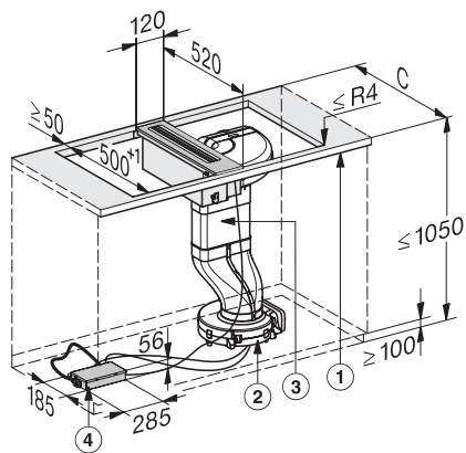
CSDA 7001 - supported installation (Skizze)
