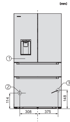
E-Com, KFFD6765 edt/cs, installation (*footnote)
