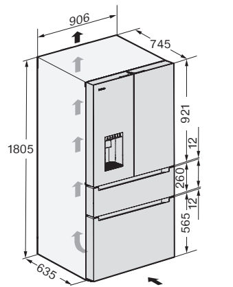
E-Com, KFFD6765 edt/cs, installation diagram
