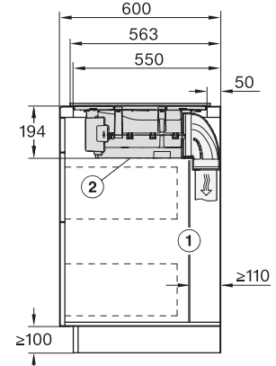
KMDA7272FR, KMDA7473FR – Side view lying on top – Installation drawing
