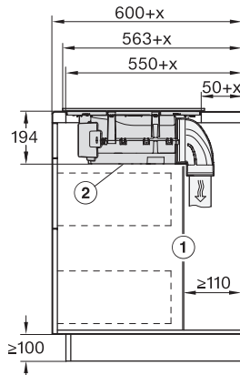
KMDA7272FR, KMDA7473FR – Side view lying on top+X – Installation drawing
