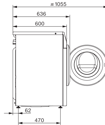
W1 drawing, slanted facade or straight facade, measures in mm
