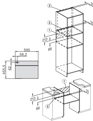
installation H7000 M, installation drawing, CH
