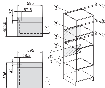
H7000 handle, glass, installation drawings
