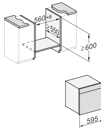
DO7860, DO7860C (CN), installation drawings
