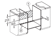
H226x-1B/BP/E/EP, H28x0B/BP, H7x6xB/BP/BPX, installation drawings - CH
