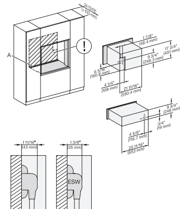
DGC7x4x+EBA7848, ESW7x70, EVS7670, Installation, 30 Zoll, Flush inset, combi, XL
