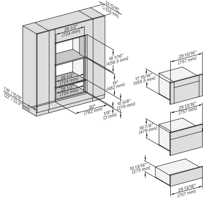
DGC7xxx+EBA7848, H7x70BM(X), ESW7x80, Einbau, 30 Zoll, Flush inset, combi, wide front, XL
