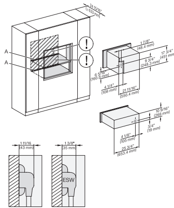
DGC7x4x+EBA7848, ESW7x80, Installation, 30 Zoll, Flush inset, combi, wide front, XL
