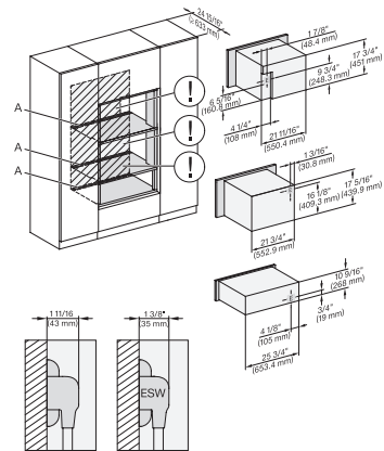
DGC7x4x+EBA7848, H7x40BM+EBA7848, ESW7x80, Installation, 30 Zoll, Flush inset, combi, XL, 450S
