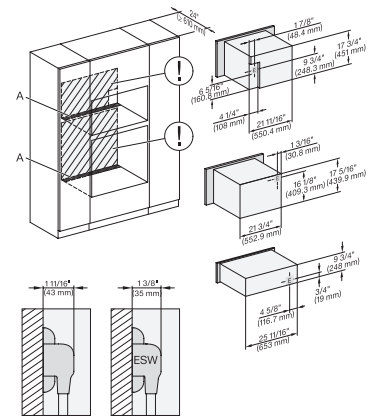
DGC7x4x+EBA7848, H7x40BM+EBA7848, ESW7x70, Installation, 30 Zoll, Proud, Flush inset, combi, XL, 450S
