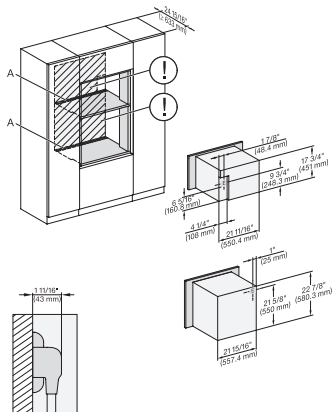
DGC7x4x(+EBA7848), H7x6xBP(+EBA7848), Installation, 30 Zol, Flush inset, combi, XL, 650S
