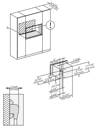
installation 30 inch Flush inset DGC XL, installation drawing, NA
