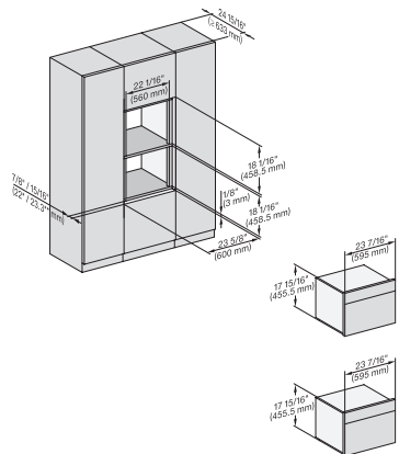
Installation Flush inset combi 450S
