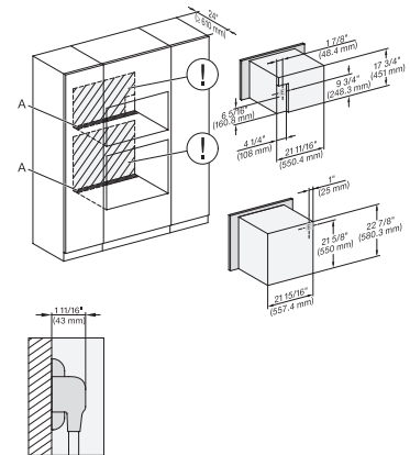
DGC7x4x(+EBA7848), H7x6x(+EBA7848), Installation, 30 Zoll, Proud, combi, XL, 650S
