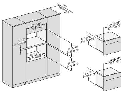
DGC7x4+EBA7848, H7x70BM, ESW7x80, Installation, 30 Zoll, Flush inset, combi, wide front, XL
