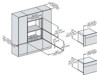
installation 30 inch Proud DGC XL, installation drawing, Na
