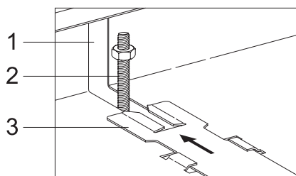
HR11xx, HR19xx, HR17xx – Installation drawing
