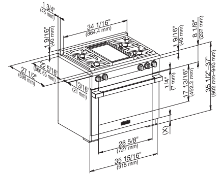
HR1936-3 (installation drawing)
