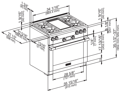
HR11xx, HR19xx, HR17xx – Installation drawing
