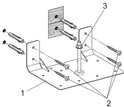
HR1136G, HR1136-1, HR1136-3 (installation drawing)
