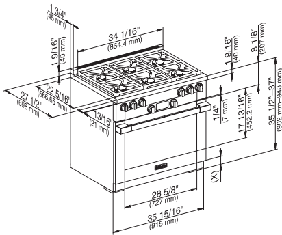
HR11xx, HR19xx, HR17xx – Installation drawing
