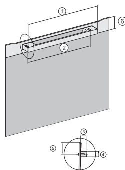
side view 30 inch Proud, installation drawing, NA
