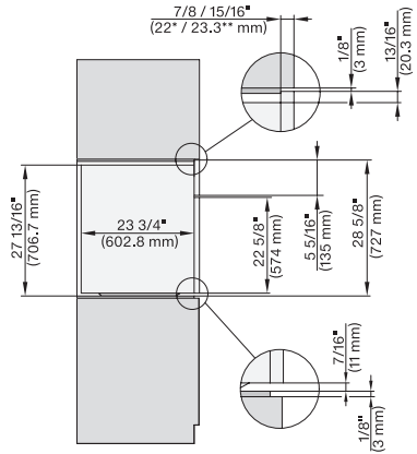
side view 30 inch Flush inset, installation drawing, NA
