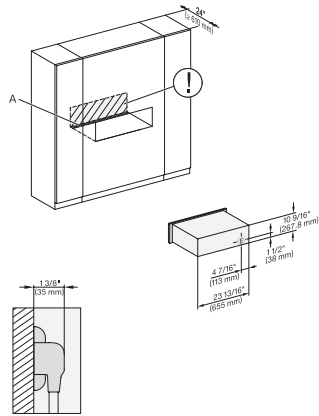
installation 30 inch Proud wide front ESW30, installation drawing, NA
